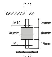
Vibration absorber
