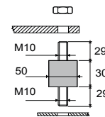
Vibration absorber
